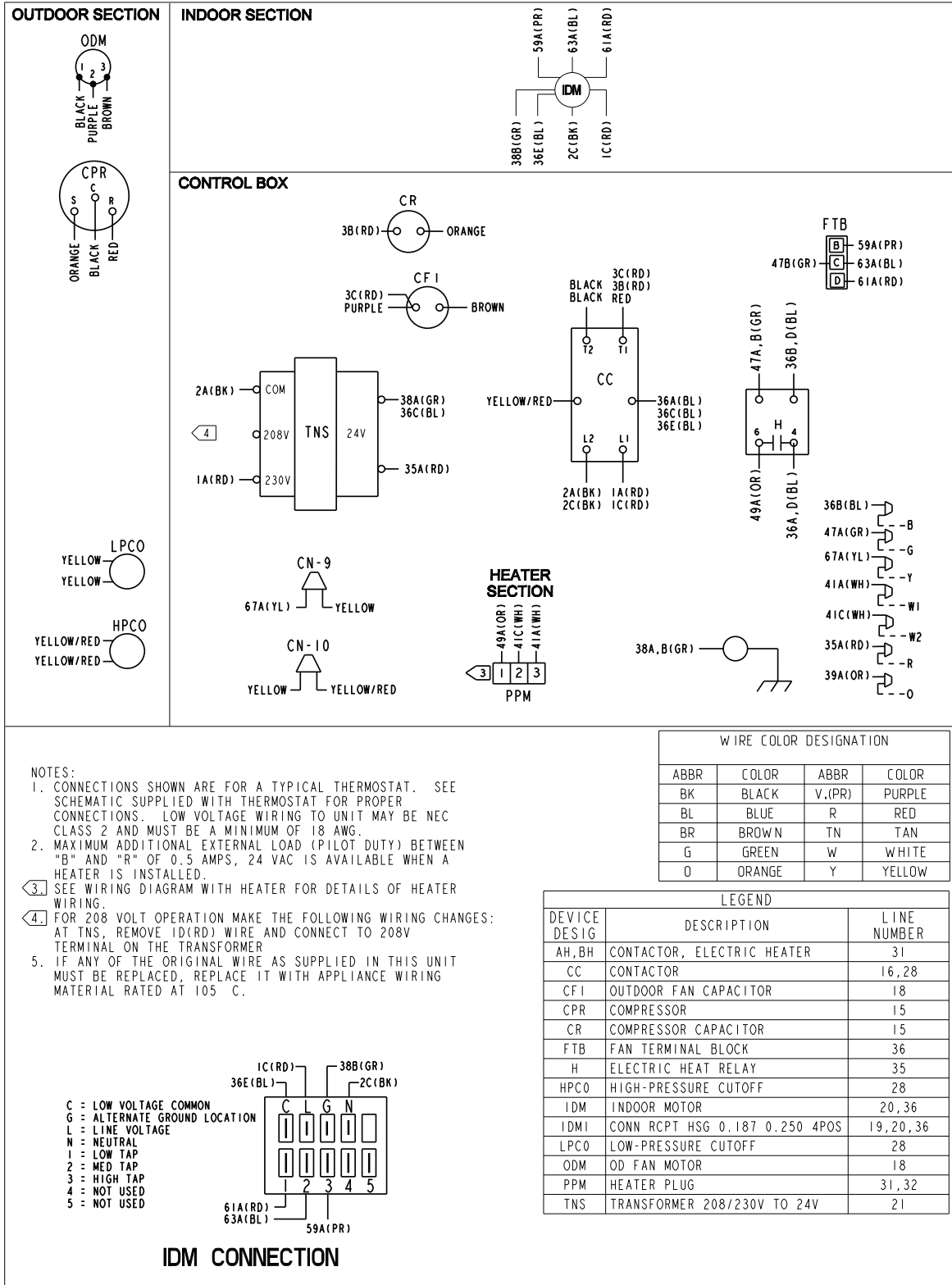
Figure 2. 4TCA4060A1 Models
