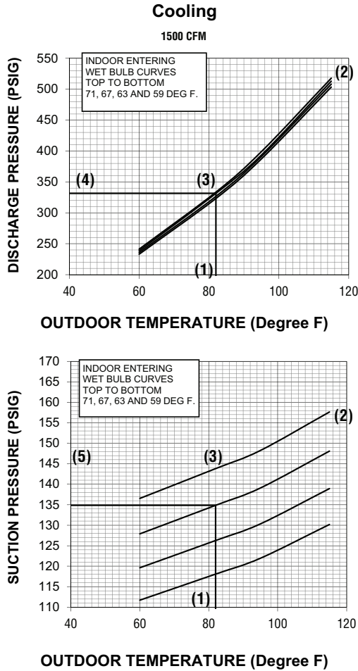
Figure 1. 4TCA4060C1
